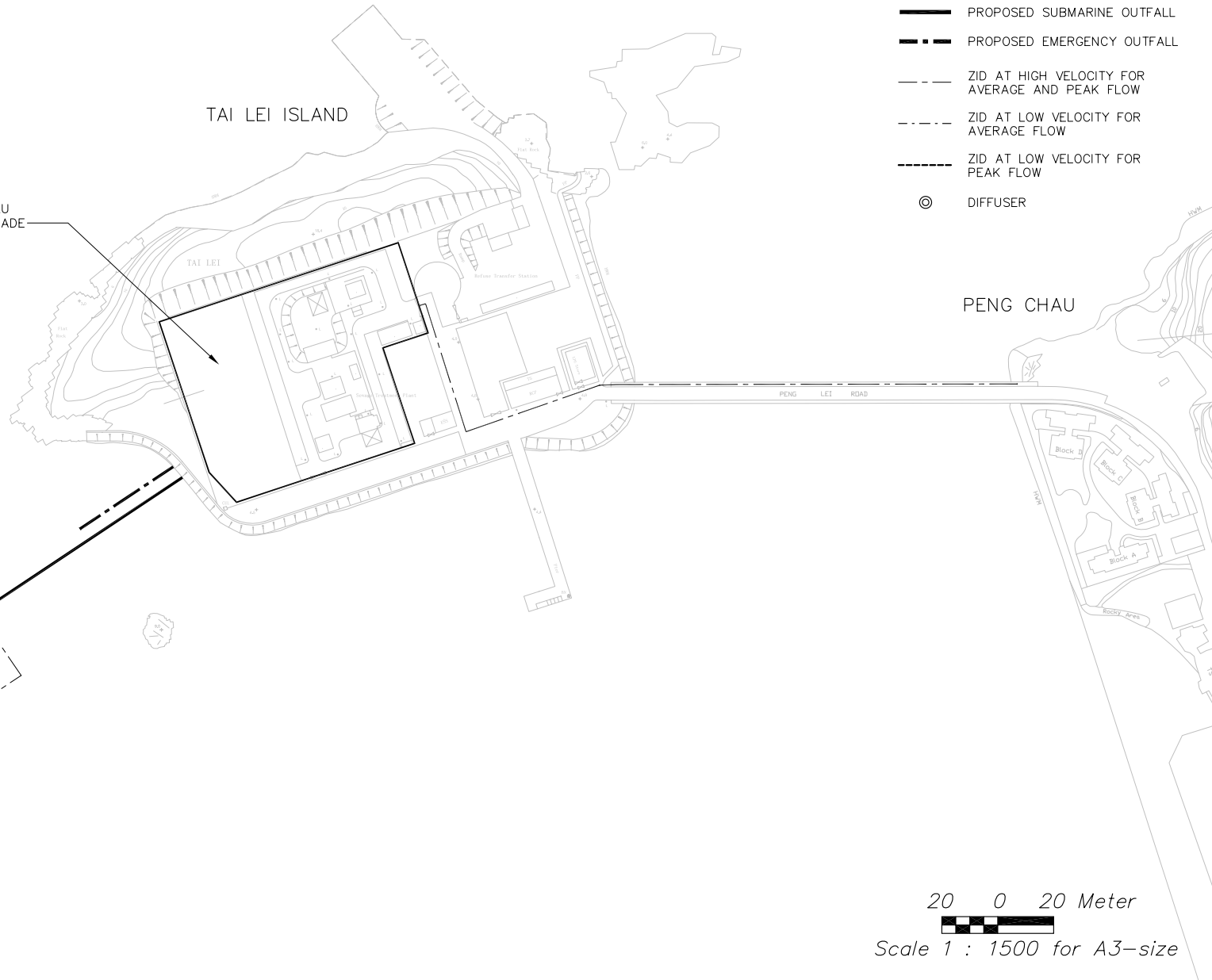
Figure 5-10 Zones of Initial Dilution (Wet Season)
